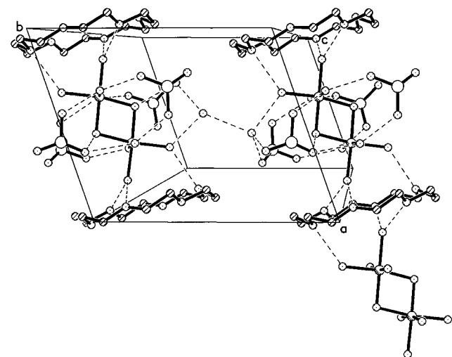
Figure 2. View of 1 showing H-bonding interactions between the dimer cation and the 18-crown-6 molecules and extending through the waters of crystallization to adjacent dimers.
