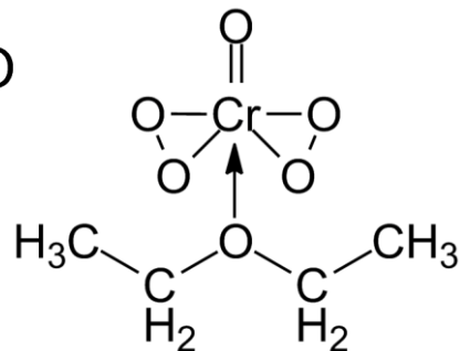
Diethyletherkomplex
