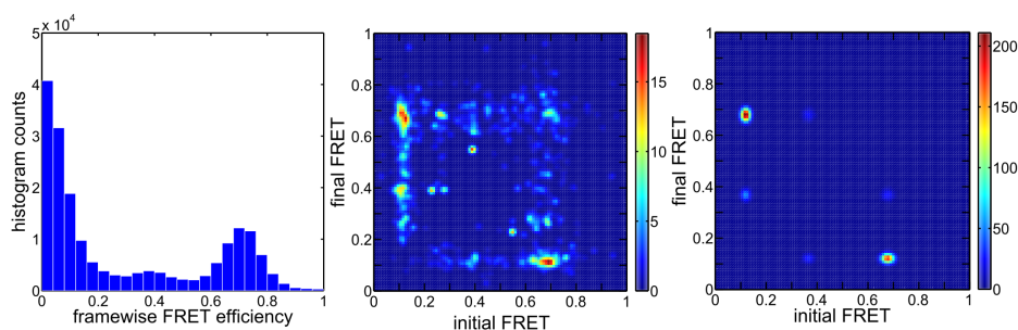
Figure 4.7: The frame-wise FRET efficiency histogram (left) for the experiments shows presence of atleast 3 FRET states. The TDP of local HMM with 3 states is shown in the middle. The TDP of global 3 state HMM is shown on the right.
