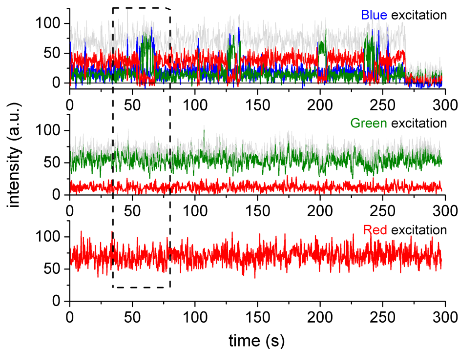
Figure 5.10: Intensity traces of a Roboarm molecule with 9 nt docking overlap and on R-G-B ALEX excitation scheme with simultaneous detection on all three cameras. Top panel: Intensity traces of all three dyes from the respective channels, upon blue excitation. Middle panel: Intensity traces of the red and green dyes from the respective channels, upon green excitation. Bottom panel: Intensity trace of red dye as detected in the red channel (camera) upon red excitation. The part of the trace highlighted in the dashed box is expanded in the figure 5.11
